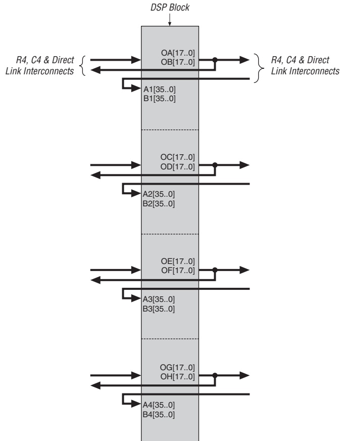
Figure 3–7. High-Level View, DSP Block Interface to Interconnect
