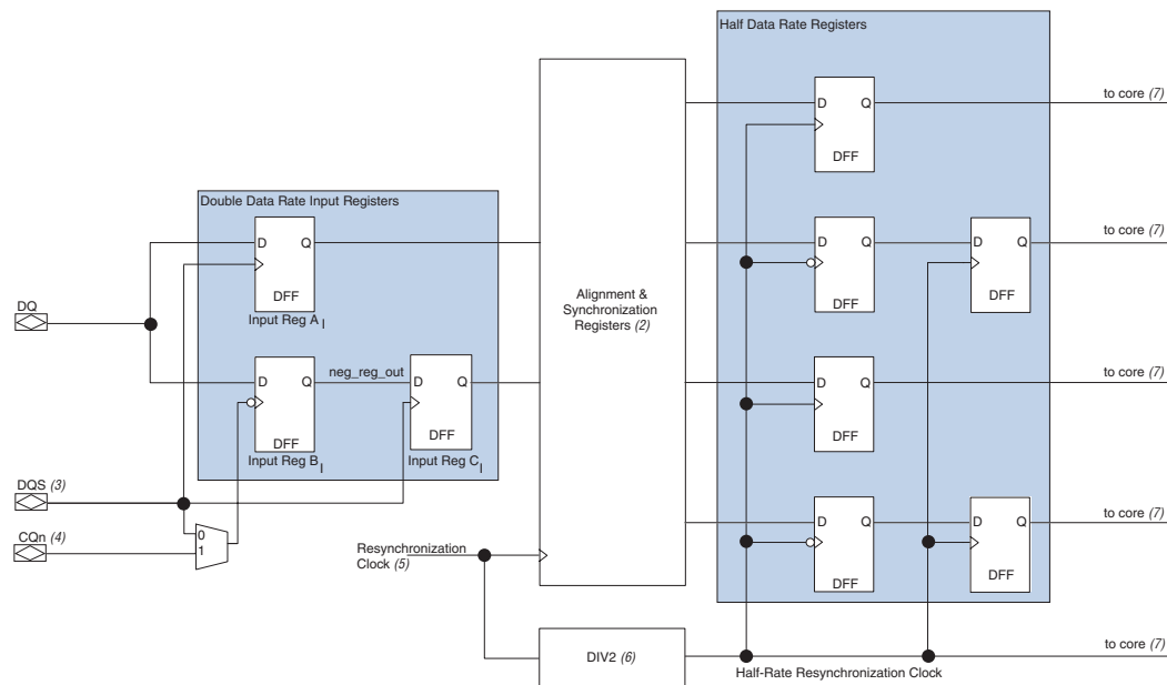
Figure 8–24. Stratix III Input Path Registers Note (1)
