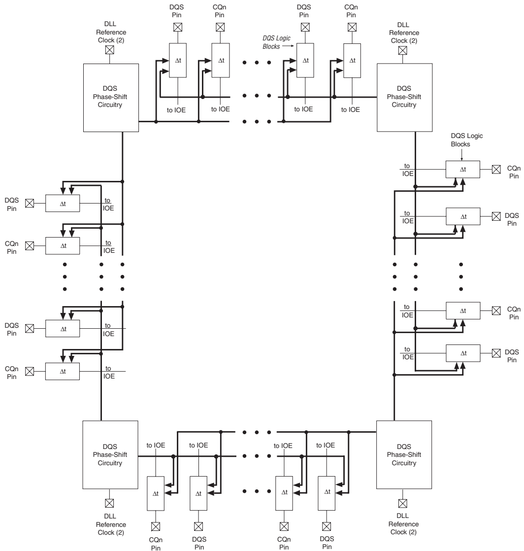
Figure 8–15. DQS & CQn Pins & DQS Phase-Shift Circuitry Note (1)
