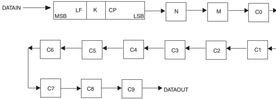
Figure 6–39. Scan-Chain Order of PLL Components for Top/Bottom PLLs Note (1)
