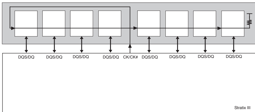
Figure 8–21. DDR3 SDRAM Unbuffered Module Clock Topology
