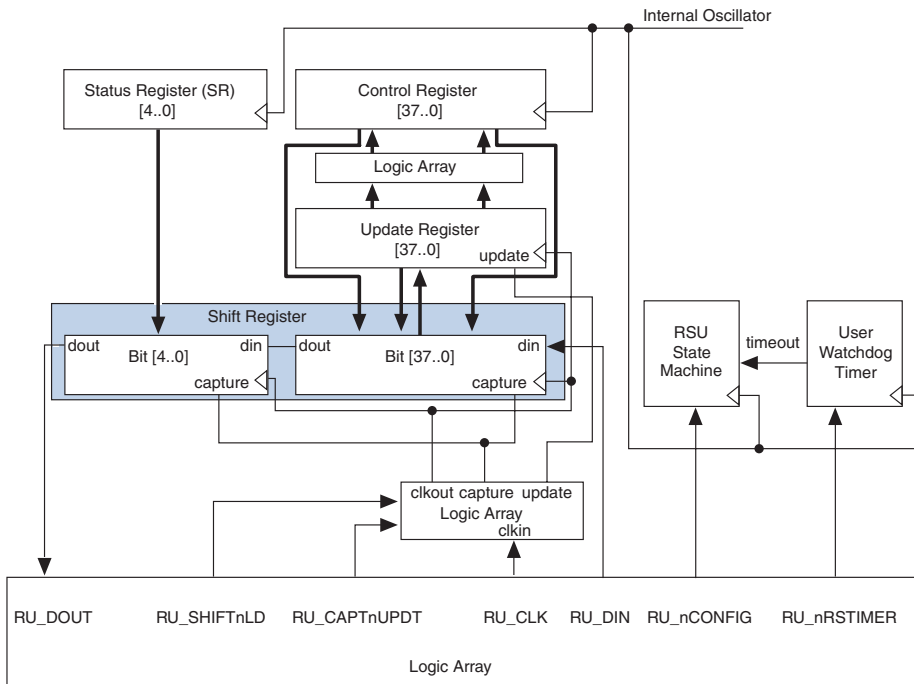
Figure 12-5. Remote System Upgrade Circuit Data Path
