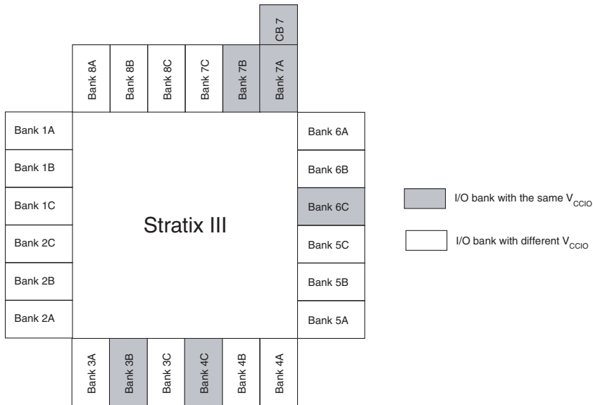
Figure 7-17. Example of Sharing Multiple I/O Banks with One OCT Calibration Block
