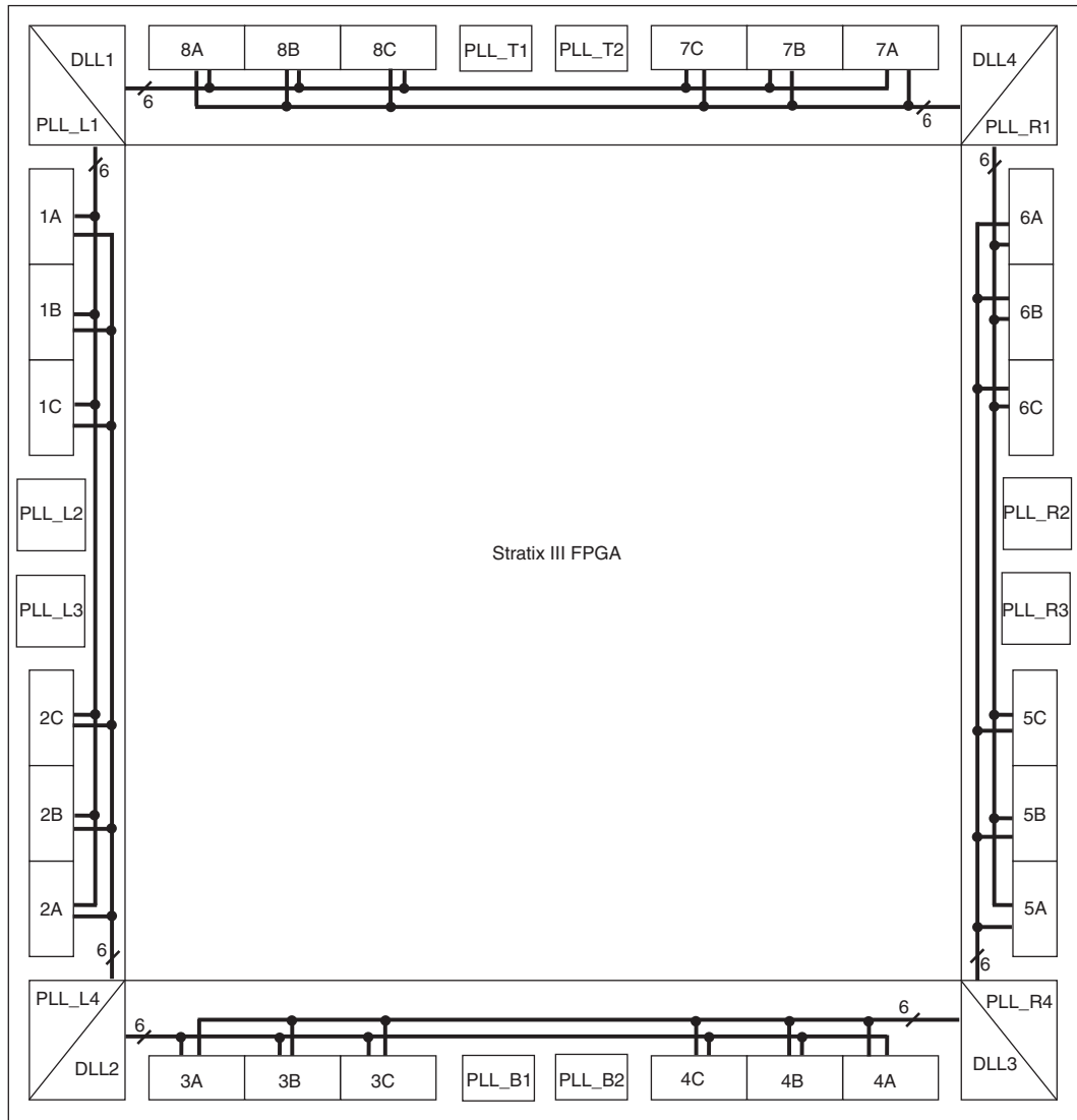
Figure 8–16. Stratix III DLL and I/O Bank Locations
