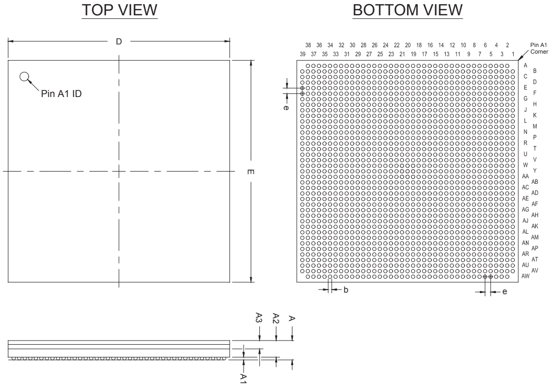
Figure 17–4. 1517-Pin Fineline Ball-Grid Array (FBGA) - Flip Chip Package Outline
