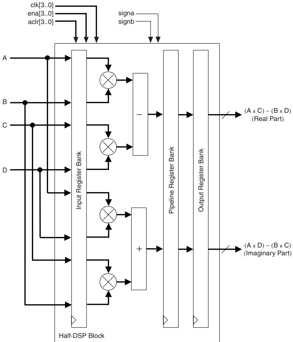
Figure 5-14. Complex Multiplier Using Two-Multiplier Adder Mode
