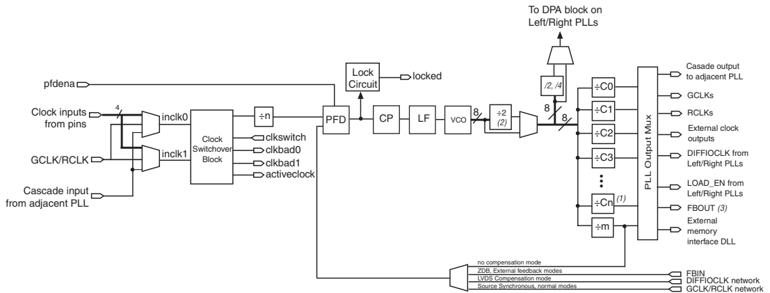
Figure 6-17. Stratix III PLL Block Diagram
