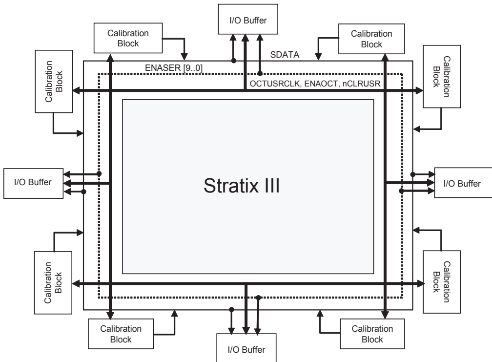
Figure 7-18. Signals for Shift-Out Codes from the OCT Calibration Block to I/O Buffers
