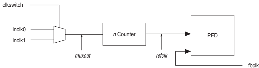
Figure 6–32. Manual Clock Switchover Circuitry in Stratix III PLLs
