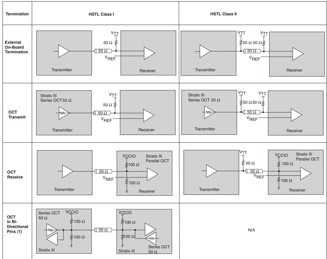
Figure 7–22. Stratix III HSTL I/O Standard Termination
