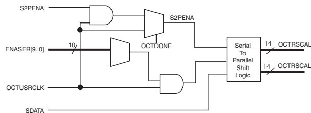
Figure 7–19. OCT Calibration Block
