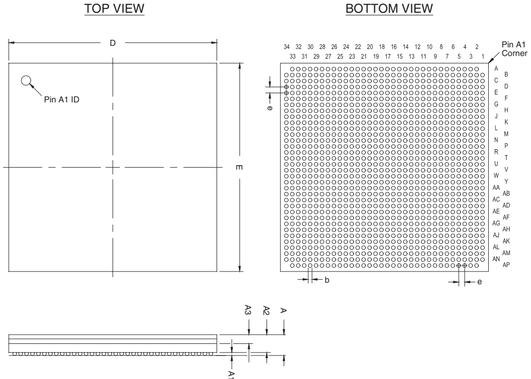
Figure 17–3. 1152-Pin FBGA Package Outline
