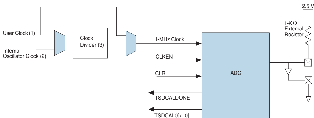
Figure 16–4. Stratix III Temperature Sensing Diode Block Diagram
