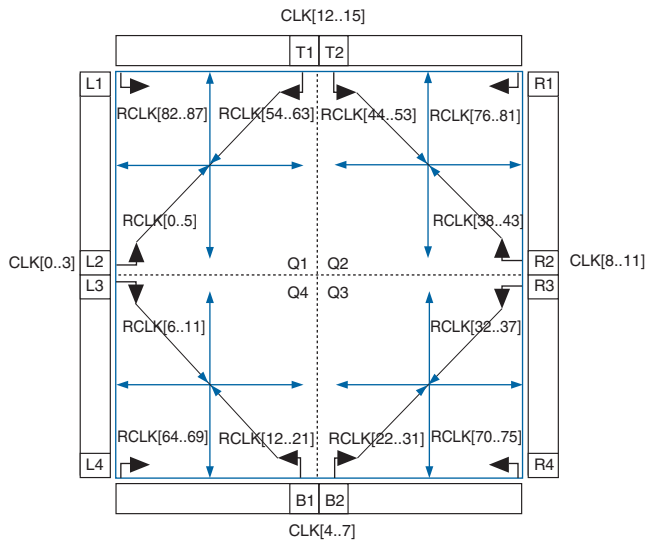
Figure 6–4. Regional Clock Networks (EP3SL200, EP3SE260, and EP3SL340 Devices)
