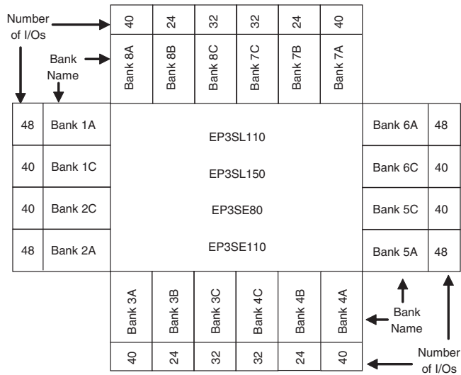
Figure 7–4. Number of I/Os in Each Bank in EP3SL110, EP3SL150, EP3SE80, and EP3SE110 Devices
