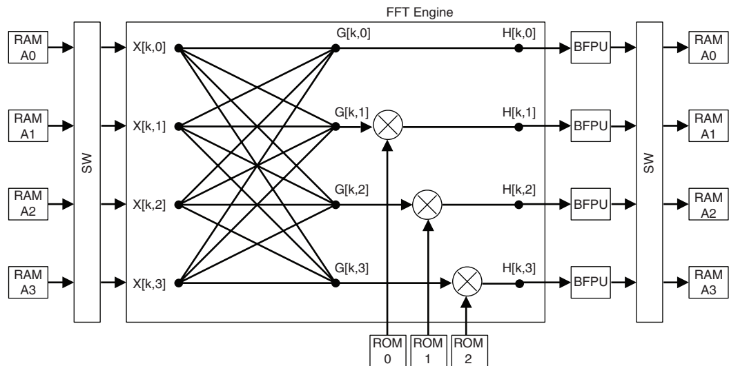
Figure 5-22. Radix-4 Butterfly
