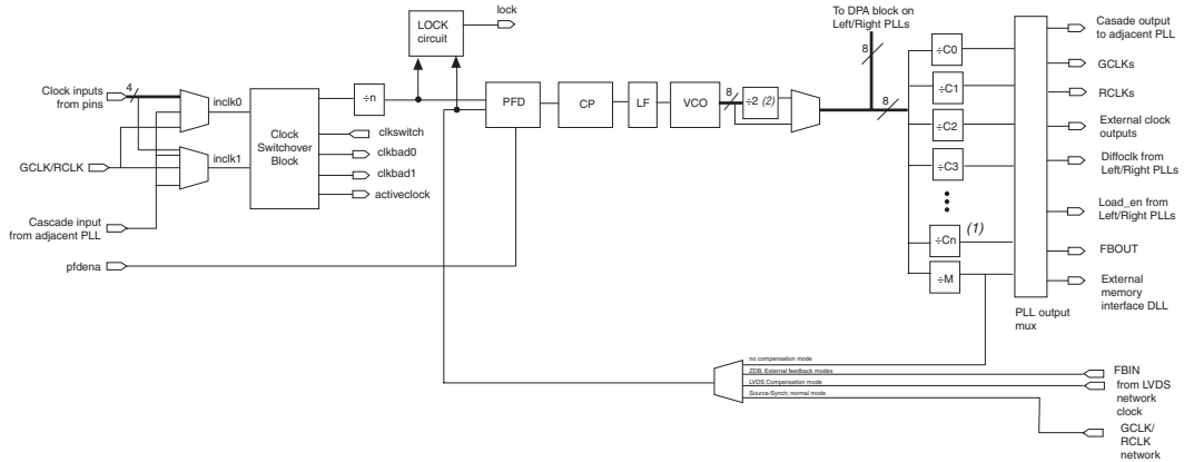
Figure 9-10. PLL Block Diagram Notes (1), (2)
