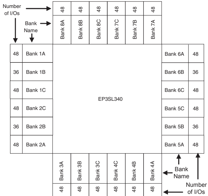
Figure 7-7. Number of I/Os in Each Bank in EP3SL340 Devices
