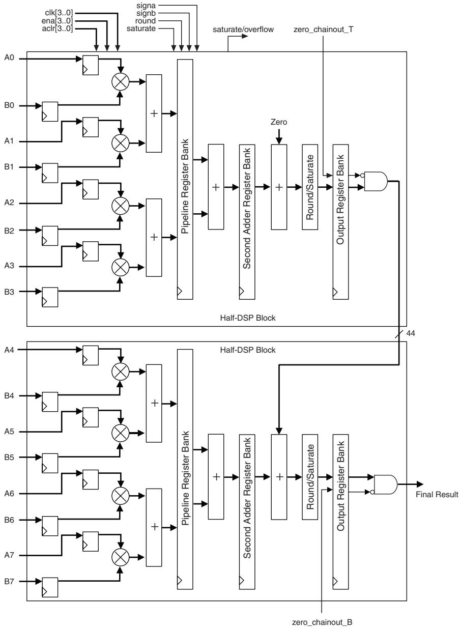
Figure 5–21. Semi-Parallel FIR Structure Using Chained Cascaded Summation
