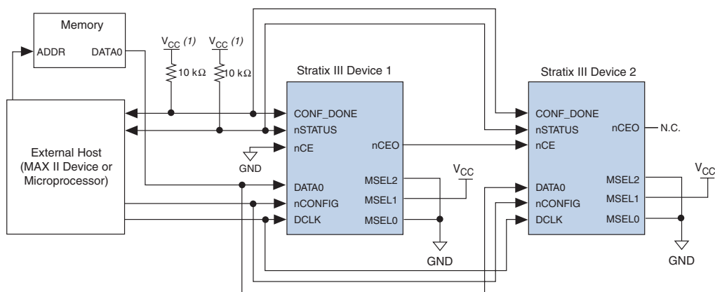
Figure 11-18. Multi-Device PS Configuration Using an External Host
