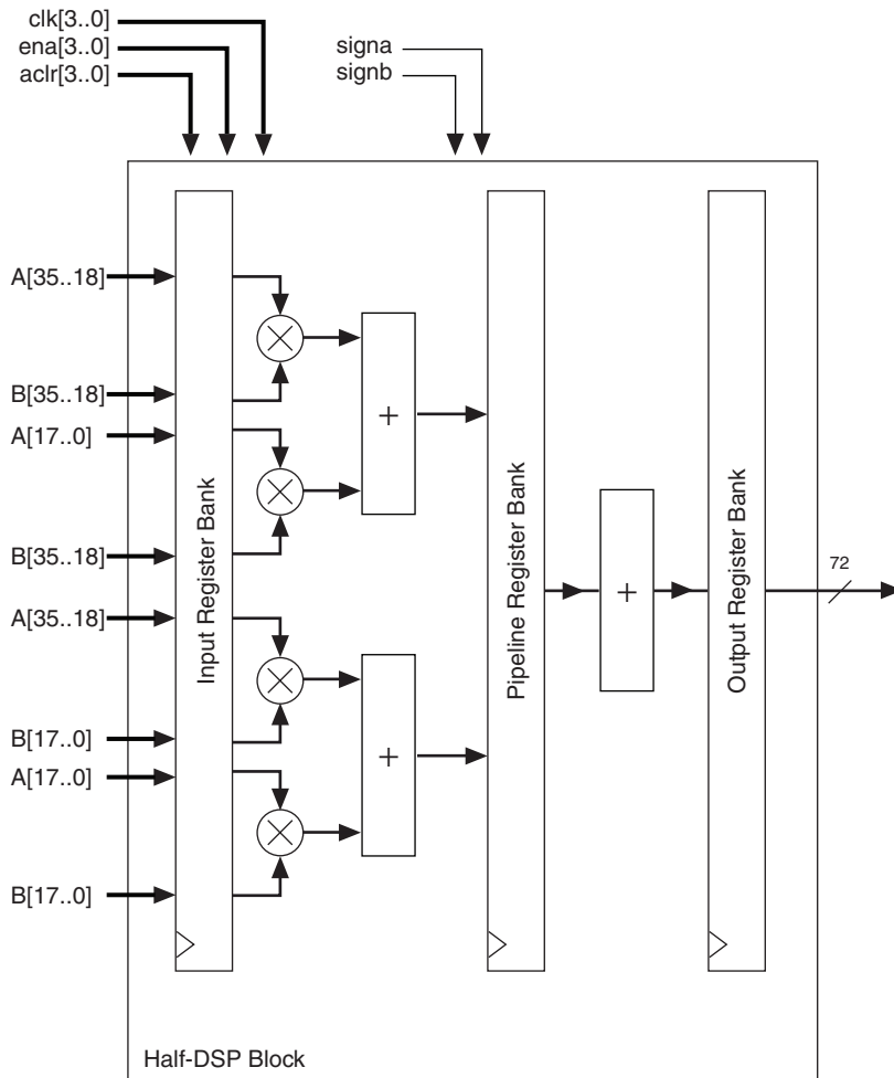
Figure 5–11. 36-Bit Independent Multiplier Mode Shown for Half-DSP Block
