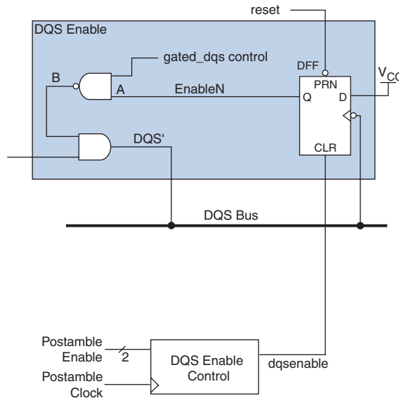
Figure 8–20. Stratix III DQS Postamble Circuitry
