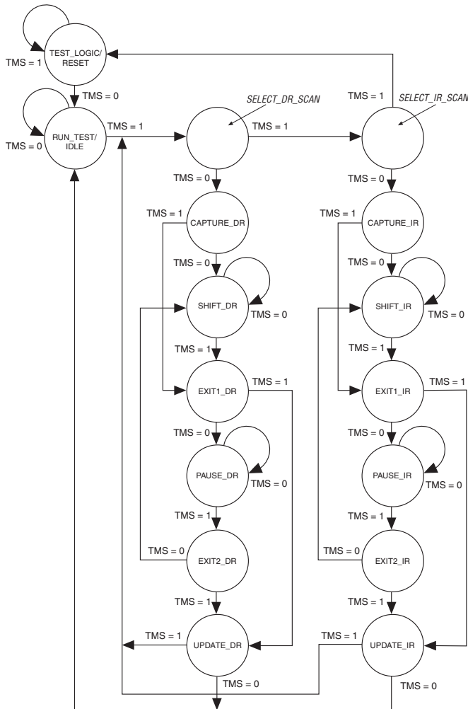
Figure 13–5. IEEE Std. 1149.1 TAP Controller State Machine
