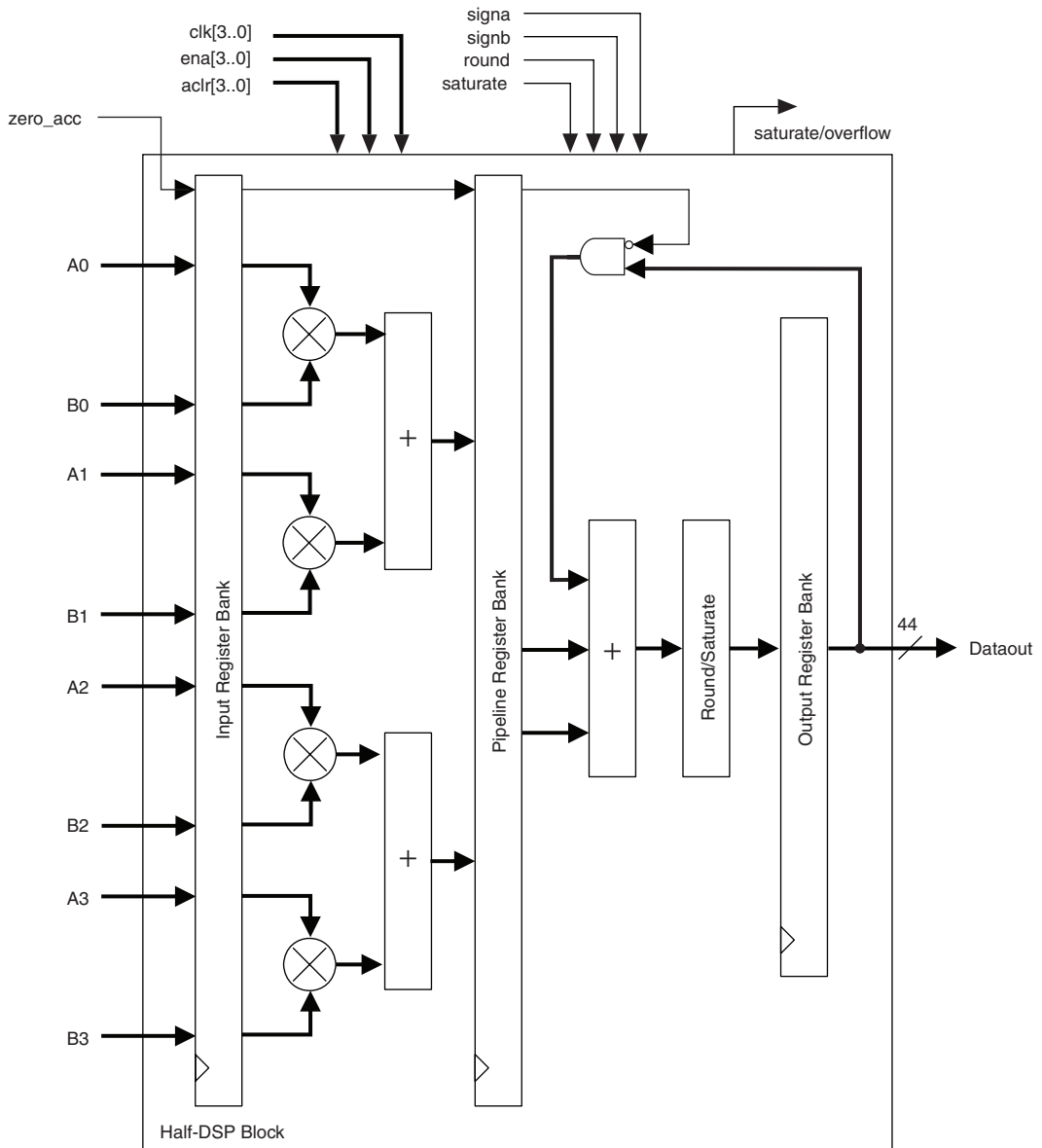
Figure 5–16. Multiply Accumulate Mode Shown for Half-DSP Block
