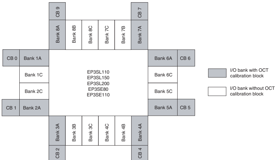
Figure 7–15. OCT Calibration Block (CB) Location in EP3SL110, EP3SL150, EP3SL200, EP3SE80, and EP3SE110 Devices
