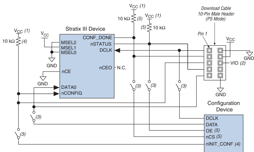
Figure 11–28. PS Configuration with a Download Cable & Configuration Device Circuit
