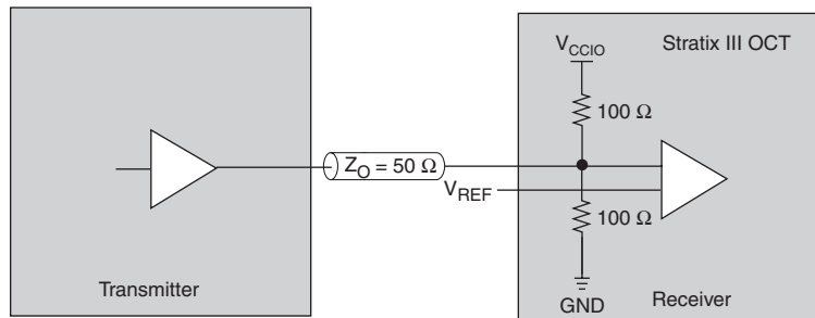
Figure 7–11. Stratix III On-Chip Parallel Termination with Calibration
