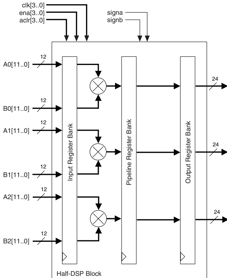
Figure 5–9. 12-Bit Independent Multiplier Mode Shown for Half-DSP Block
