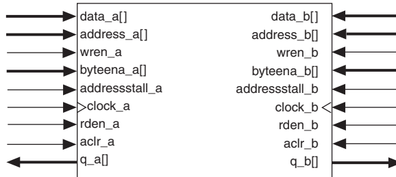
Figure 4-12. Stratix III True Dual-Port Memory Note (1)
