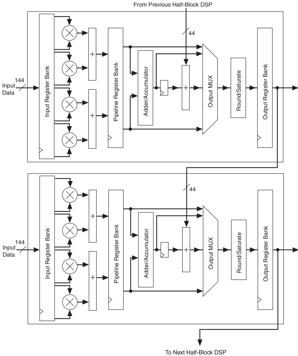
Figure 5–5. Stratix III Full DSP Block Summary
