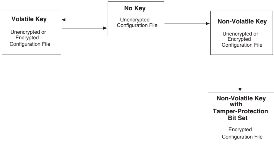
Figure 14–2. Stratix III Security Modes - Sequence & Restrictions
