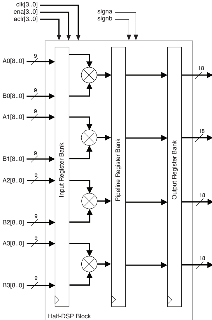
Figure 5–10. 9-Bit Independent Multiplier Mode Shown for Half-Block
