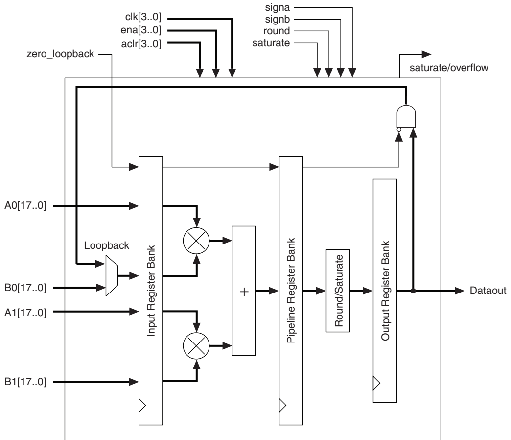
Figure 5-13. Loopback Mode for Half-DSP Block
