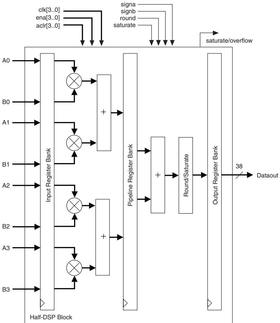
Figure 5–15. Four-Multiplier Adder Mode Shown for Half-DSP Block
