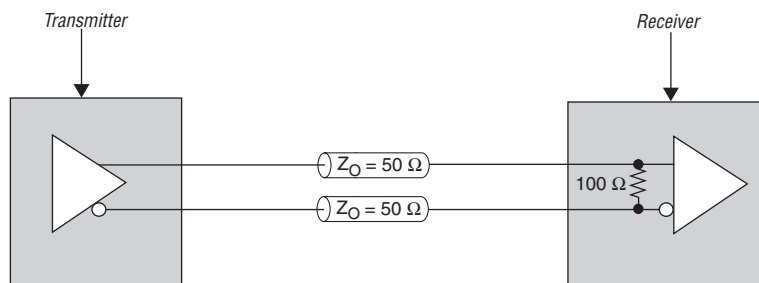
Figure 7-13. Differential Input On-Chip Termination
