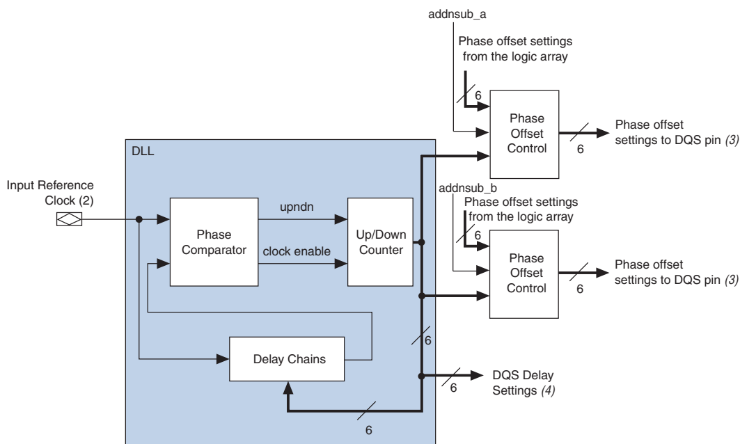
Figure 8–17. Simplified Diagram of the DQS Phase Shift Circuitry Note (1)
