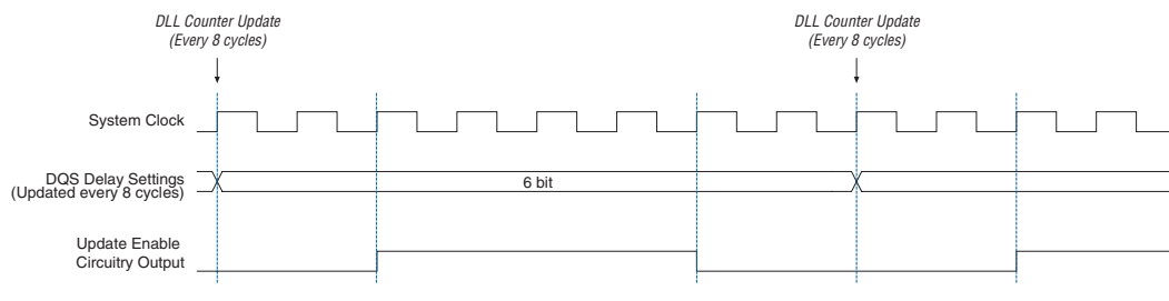
Figure 8–19. DQS Update Enable Waveform
