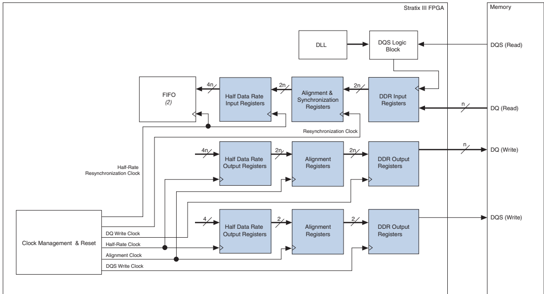
Figure 8–2. External Memory Interface Data Path Overview Note (1)
