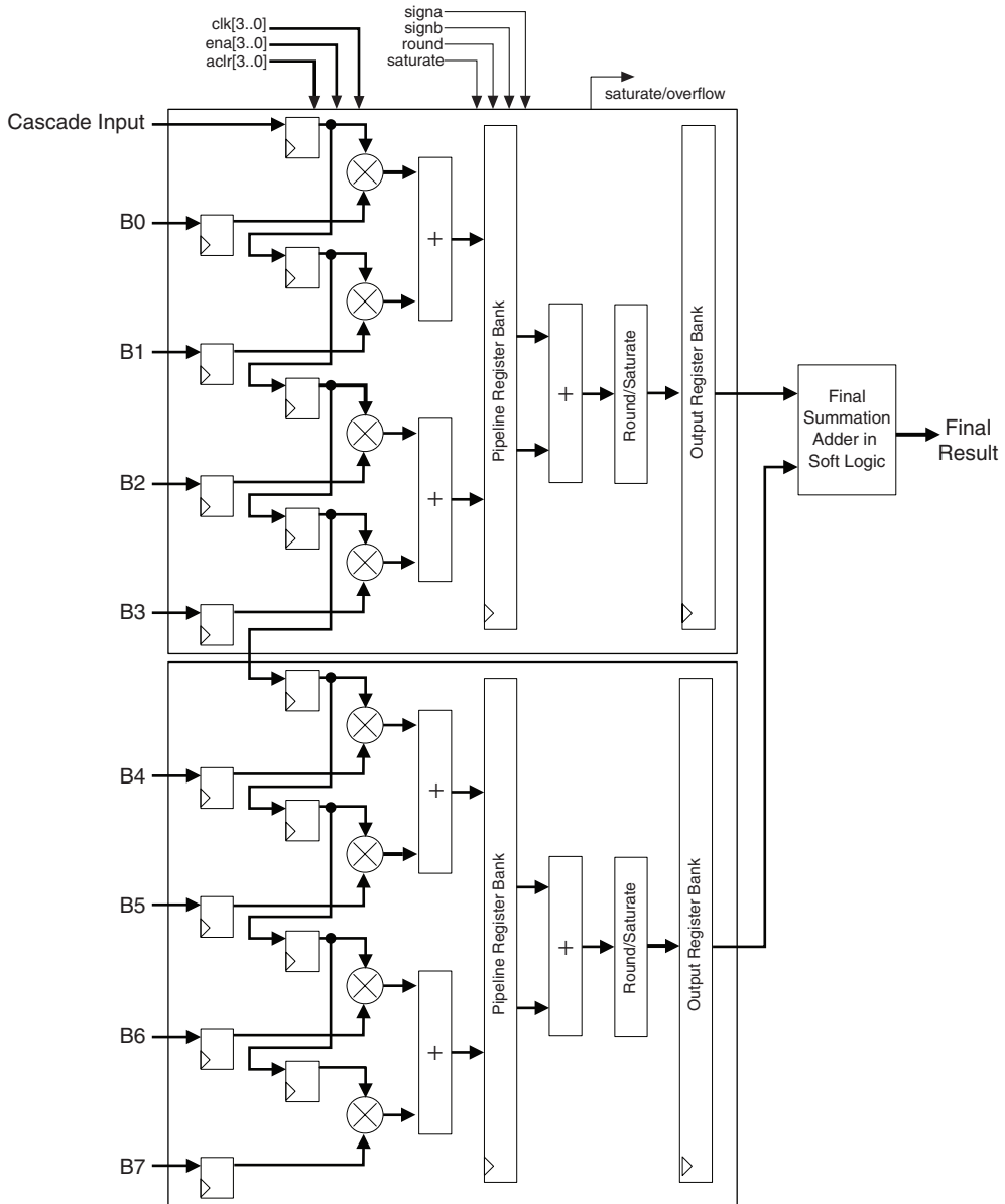
Figure 5–19. FIR Filter Using Tap-Delay Line Input & Tree Summation of Final Result
