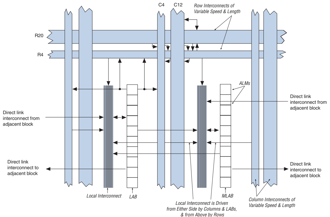
Figure 2–1. Stratix III LAB Structure
