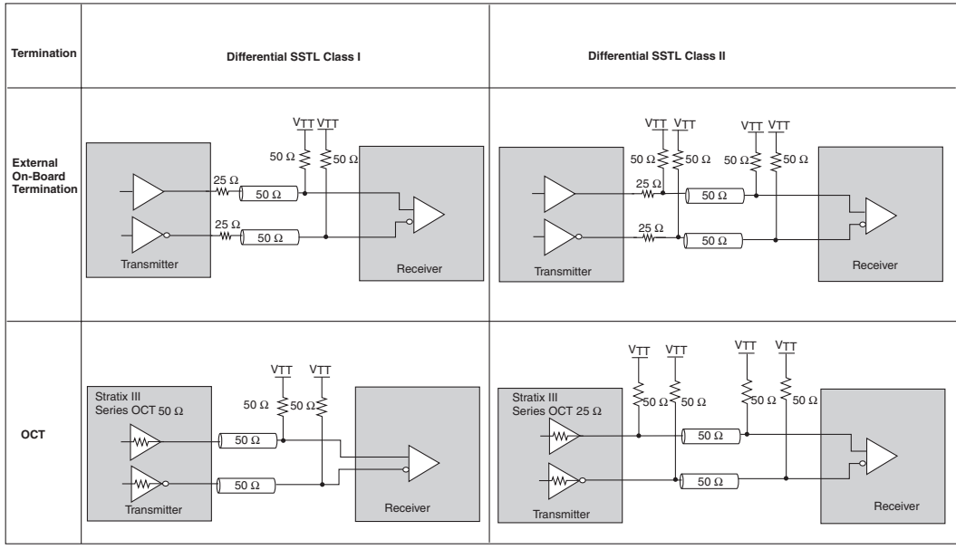
Figure 7–23. Stratix III Differential SSTL I/O Standard Termination
