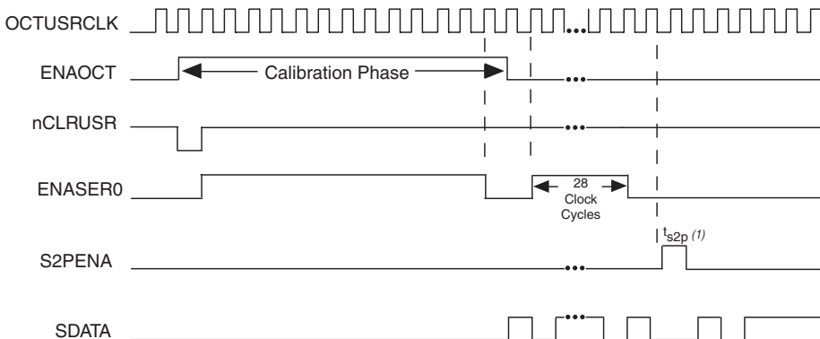
Figure 7–20. OCT User-Mode Signal Timing Waveform
