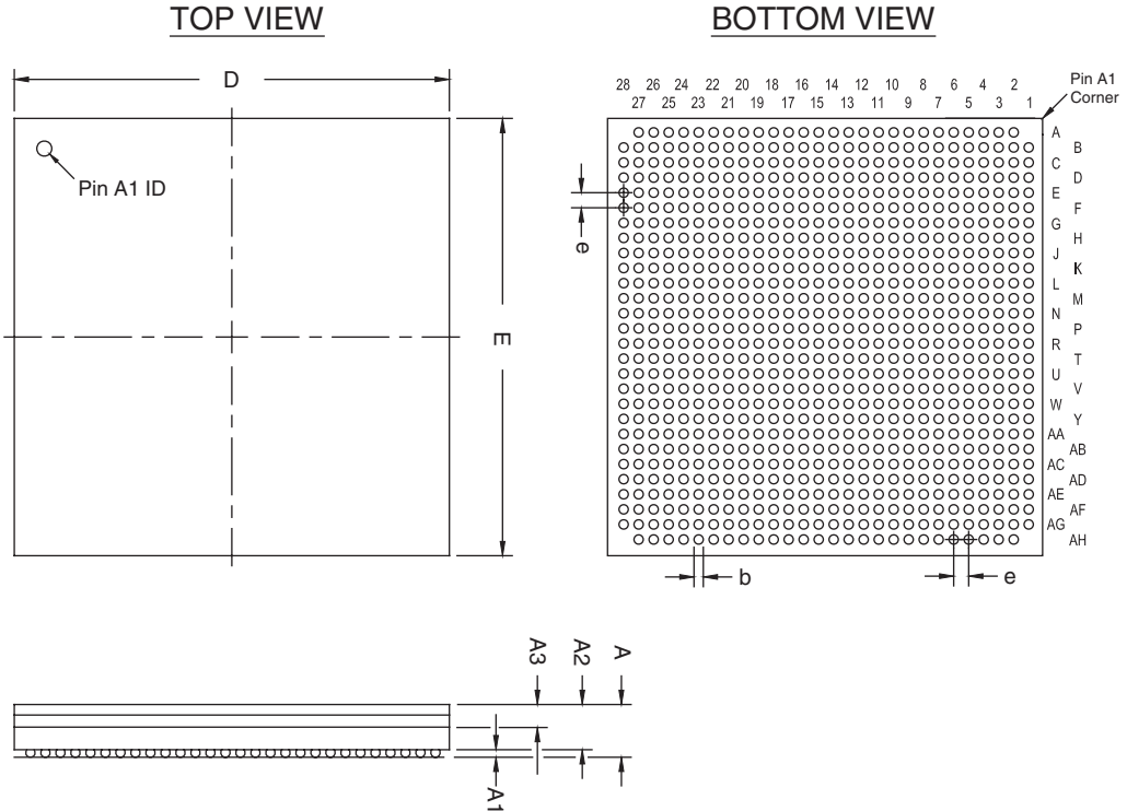
Figure 17-2. 780-Pin FBGA Package Outline
