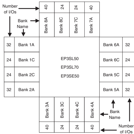
Figure 7–3. Number of I/Os in Each Bank in EP3SL50, EP3SL70, and EP3SE50 Devices
