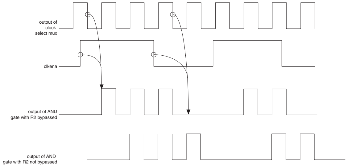
Figure 6–15. clkena Signals
