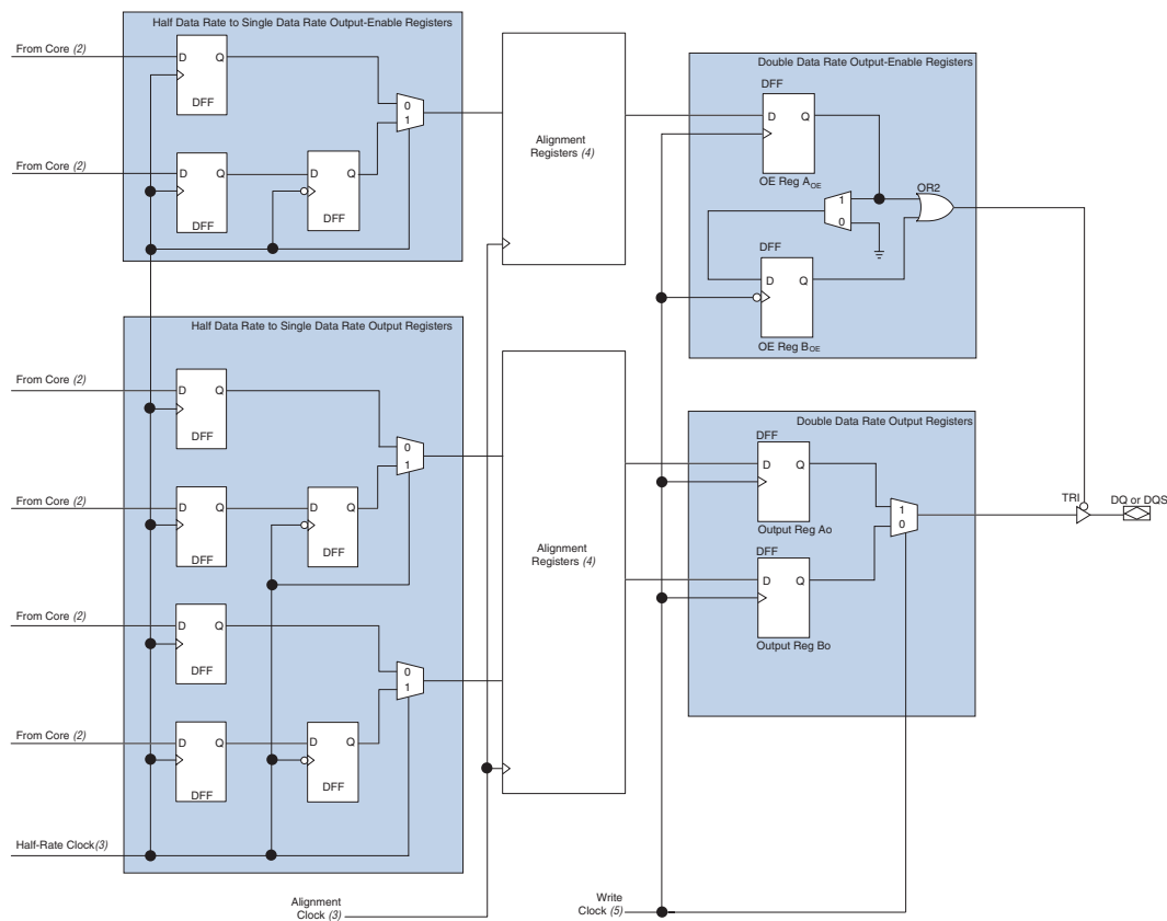
Figure 8–25. Stratix III Output & Output-Enable Path Registers Note (1)
