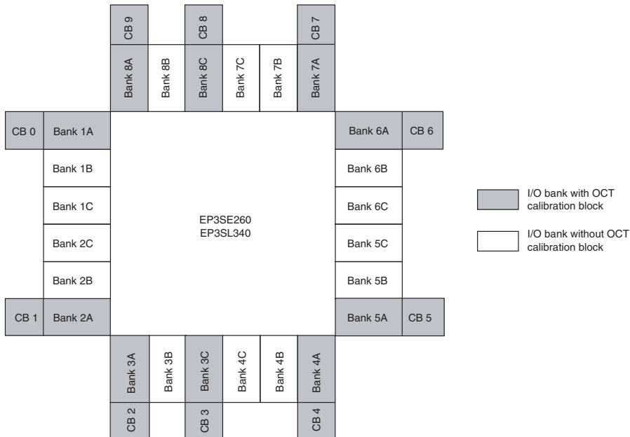
Figure 7–16. OCT Calibration Block (CB) Location in EP3SE260 and EP3SL340
