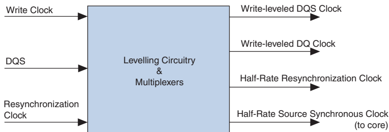
Figure 8–22. Stratix III Read & Write Leveling Delay Chains & Multiplexers
