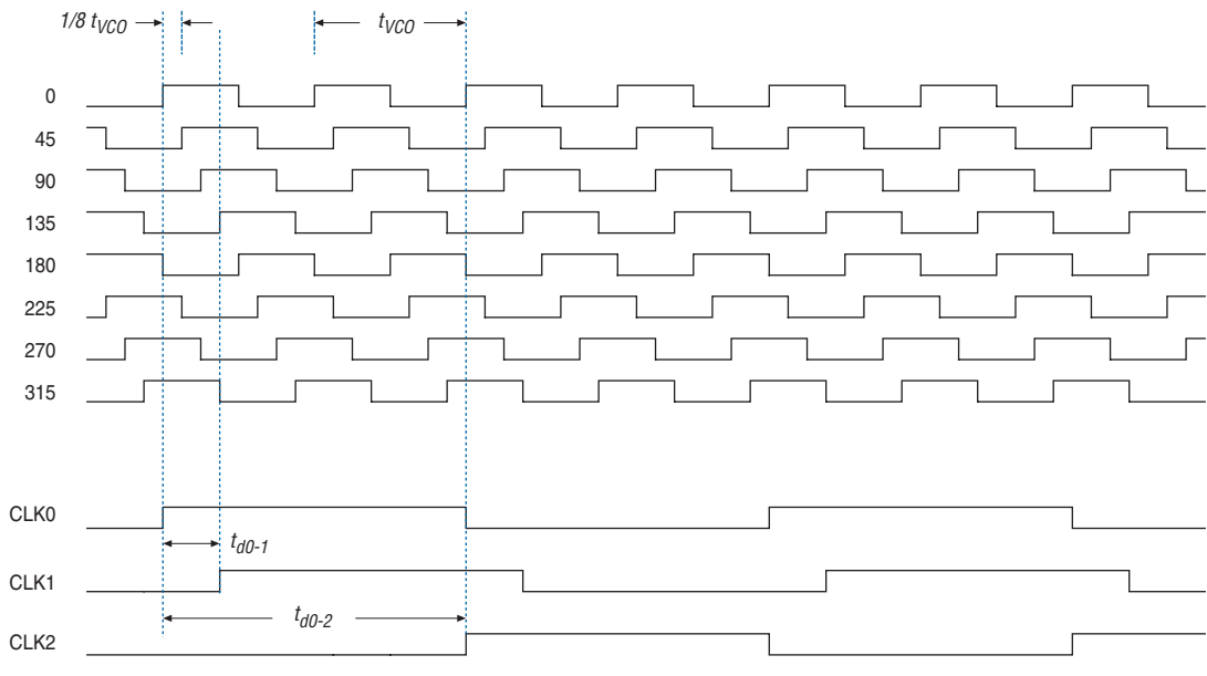
Figure 6–36. Delay Insertion Using VCO Phase Output & Counter Delay Time
