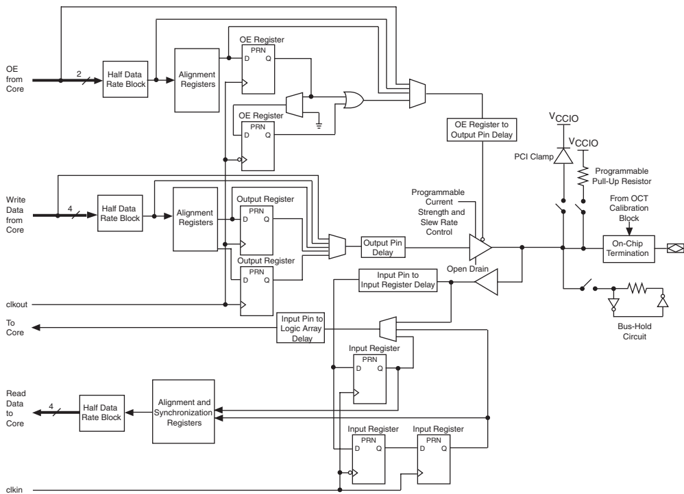
Figure 7–8. Stratix III IOE Structure
