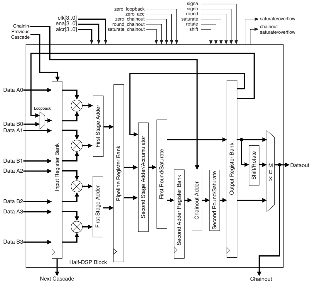
Figure 5–6. Half-DSP Block Architecture
