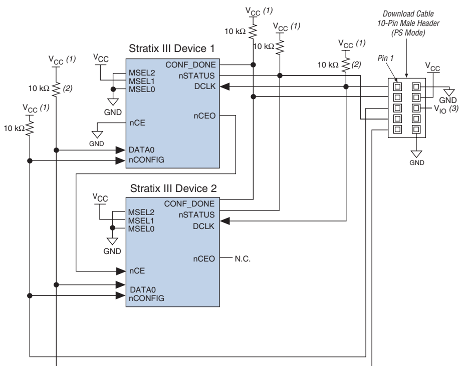
Figure 11–27. Multi-Device PS Configuration using a USB Blaster, MasterBlaster, ByteBlaster II or ByteBlasterMV Cable
