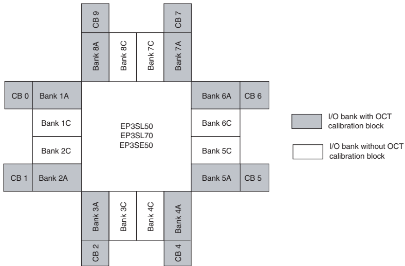
Figure 7–14. OCT Calibration Block (CB) Location in EP3SL50, EP3SL70, and EP3SE50 Devices
