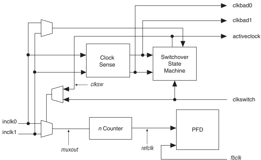
Figure 6–29. Automatic Clock Switchover Circuit Block Diagram
