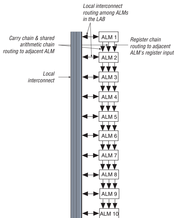
Figure 2–18. Shared Arithmetic Chain, Carry Chain, & Register Chain Interconnects
