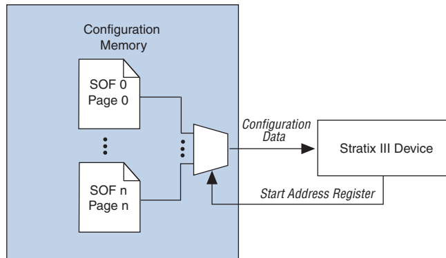
Figure 12–3. Page Mode Operation in a Stratix III Device
