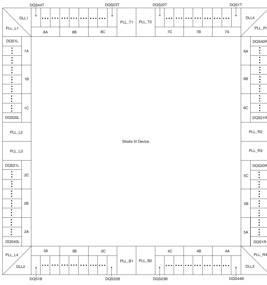
Figure 8–13. DQS Pins in Stratix III I/O Banks
