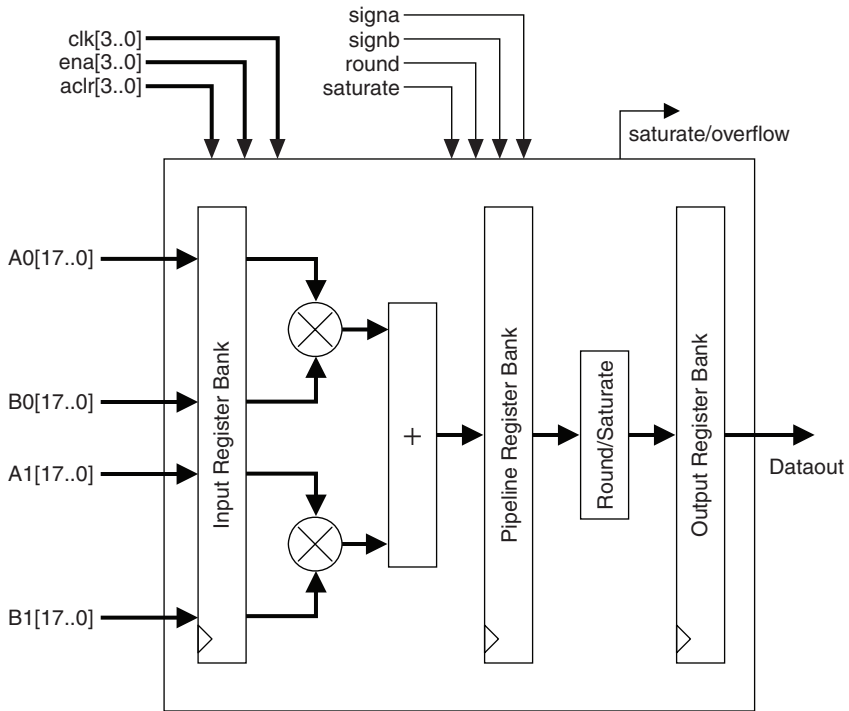
Figure 5–12. Two-Multiplier Adder Mode Shown for Half-DSP Block
