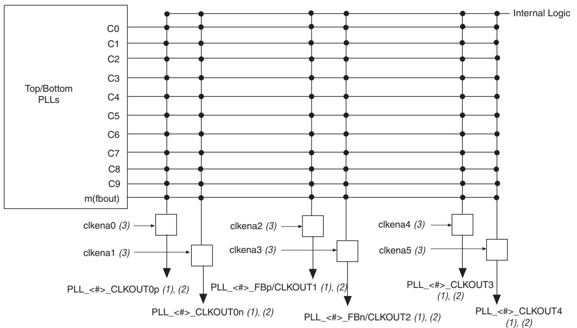
Figure 6–18. External Clock Outputs for Top/Bottom PLLs
