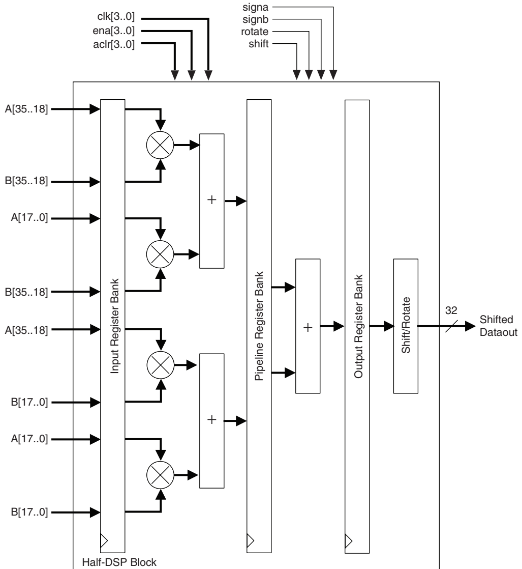
Figure 5-17. Shift Operation Mode Shown for Half-DSP Block
