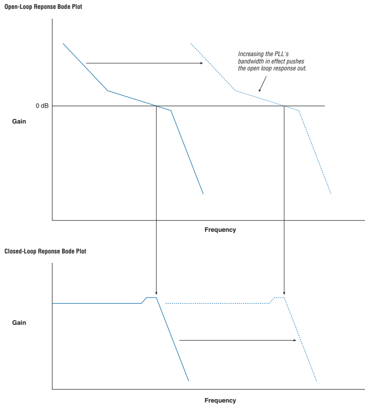
Figure 6–34. Open- & Closed-Loop Response Bode Plots
