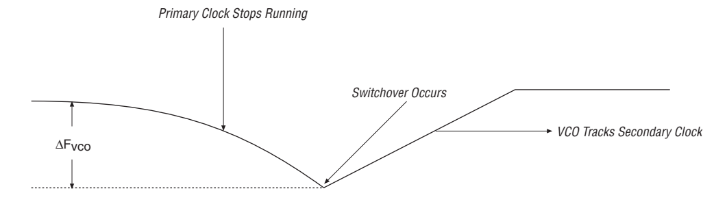
Figure 6–33. VCO Switchover Operating Frequency
