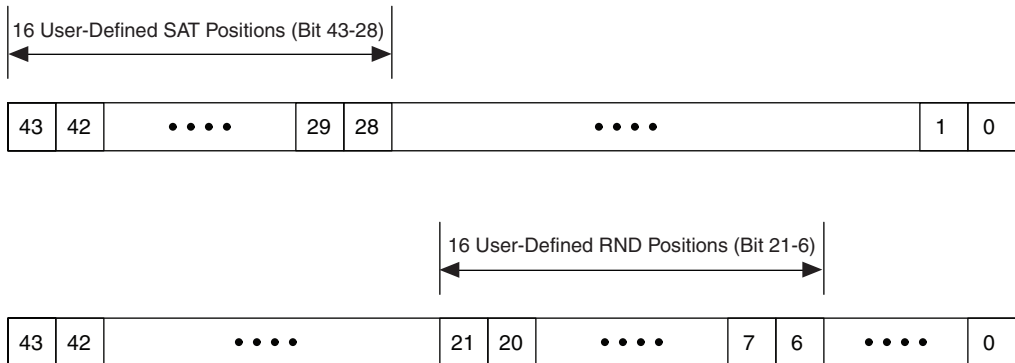
Figure 5–18. Round and Saturation Locations
