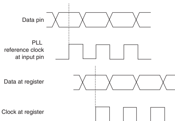
Figure 6–21. Phase Relationship Between Clock & Data in Source-Synchronous & LVDS Modes
