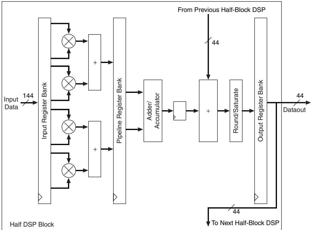
Figure 5–4. Output Cascading Feature for FIR Structures
