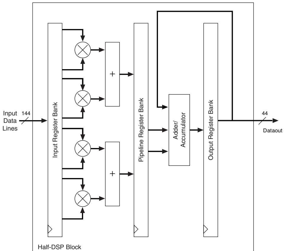
Figure 5–3. Four-Multiplier Adder &amp; Accumulation Capability
