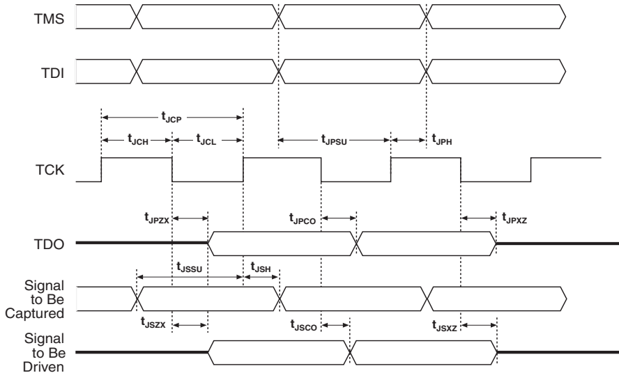
Figure 13–6. IEEE Std. 1149.1 Timing Waveforms
