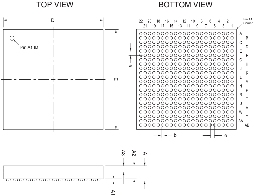
Figure 17-1. 484-Pin FBGA Package Outline
