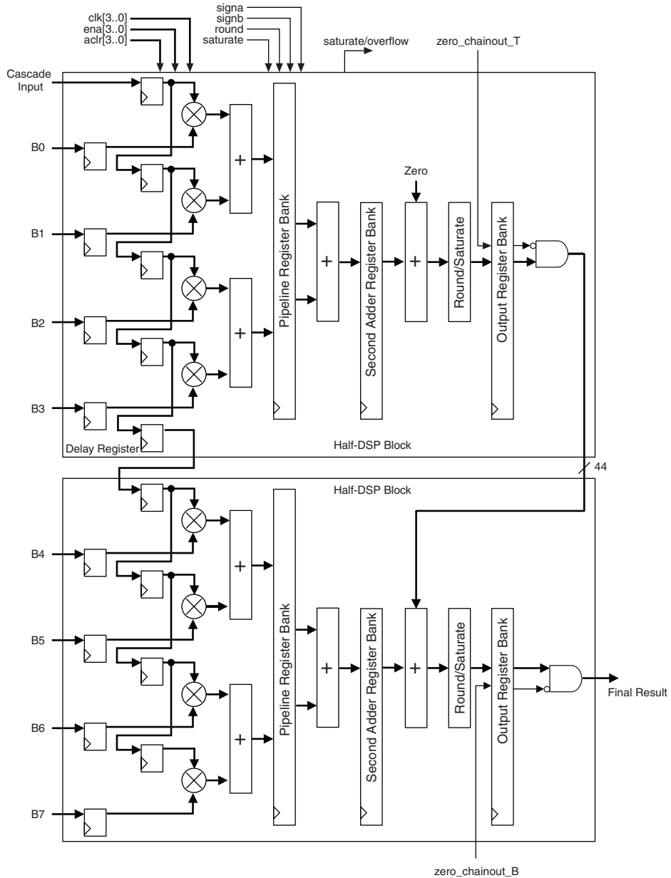
Figure 5–20. FIR Filter using Tap-Delay Line Input & Chained Cascade Summation of Final Result
