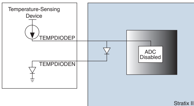
Figure 16-3. Connections When ADC is Bypassed
