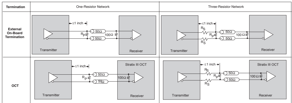
Figure 7-29. Stratix III mini-LVDS I/O Standard Termination Note (1)
