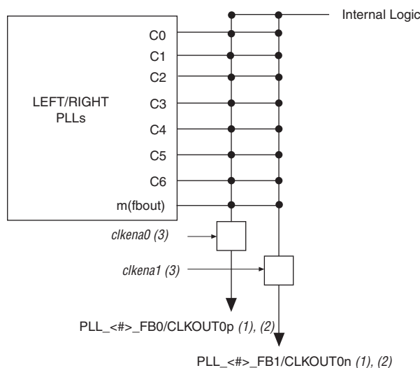
Figure 6–19. External Clock Outputs for Left/Right PLLs
