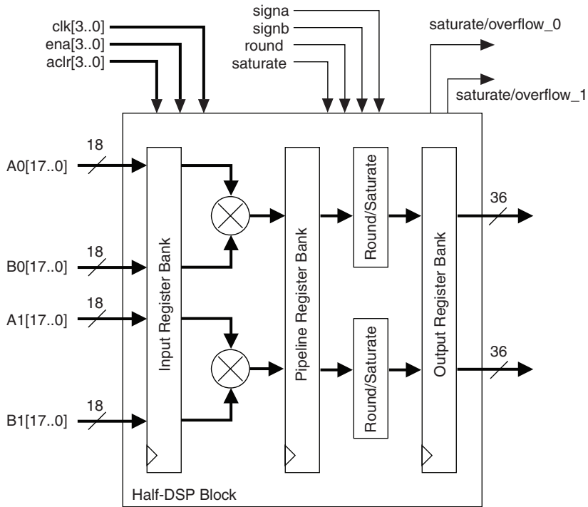
Figure 5–8. 18-Bit Independent Multiplier Mode Shown for Half-DSP Block
